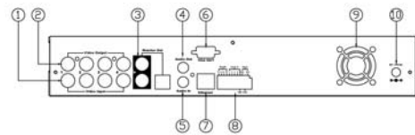
Back Panel Layout
